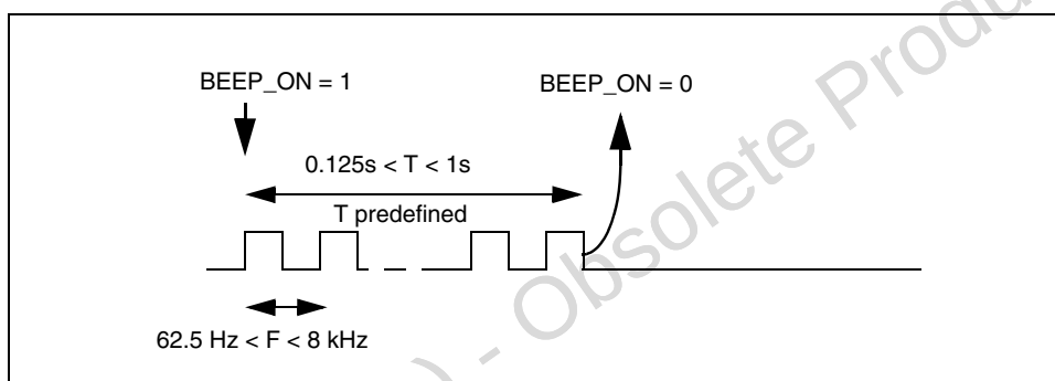
Figure 13: Pulse Mode
